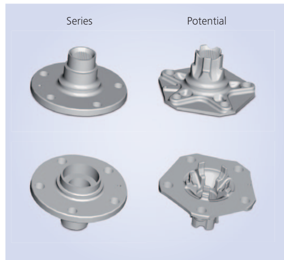
Figure 38: Wheel bearing – Comparison of the series part and the lightweight design proposal
