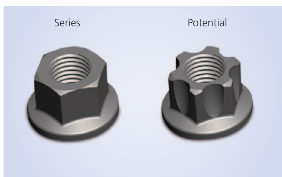
Figure 41: Hexagon nut with flange and following weight optimisation
